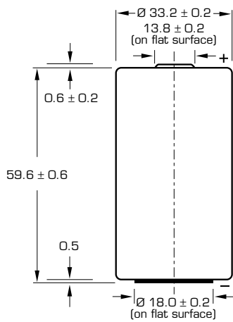
Finished version with flat positive end cap
