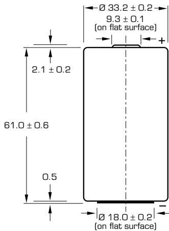
Finished version with protruding positive end cap
